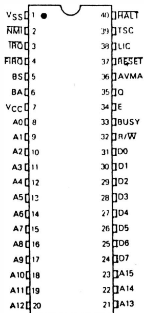
FIGURE 1 - PIN ASSIGNMENT
